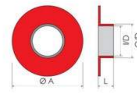
TYPE SFR WITH ROUND FLANGE
