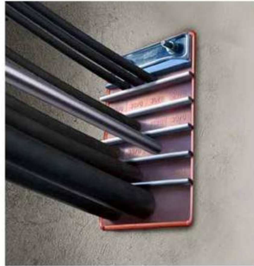
Casting into concrete RGB transit
